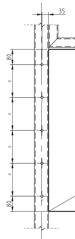
DETAIL B SCALE 1:10
